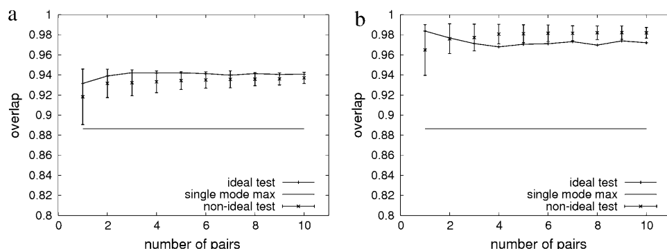
FIGURE 4 Summary of results for transition (2lao \rightarrow 1lst). Panel a shows the overlap between the computed and the measured conformational changes versus the number of pairwise distance constraints. Panel b shows the overlap between the computed conformational change and mode No. 1 versus the number of pairwise distance constraints. Line with pluses, result for the ideal test; horizontal line, the maximal overlap between any single mode and the measured conformational change; x-marks with error bars, result for the nonideal test 1, where the error bar shows 1 SD.
