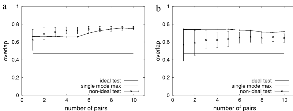
FIGURE 3 Summary of results for transition (1ypt → 1yts). Panel a shows the overlap between the computed and the measured conformational changes versus the number of pairwise distance constraints. Panel b shows the overlap between the computed conformational change and mode No. 6 versus the number of pairwise distance constraints. Line with pluses, result for the ideal test; horizontal line, the maximal overlap between any single mode and the measured conformational change; x-marks with error bars, result for the nonideal test 1, where the error bar shows 1 SD.
