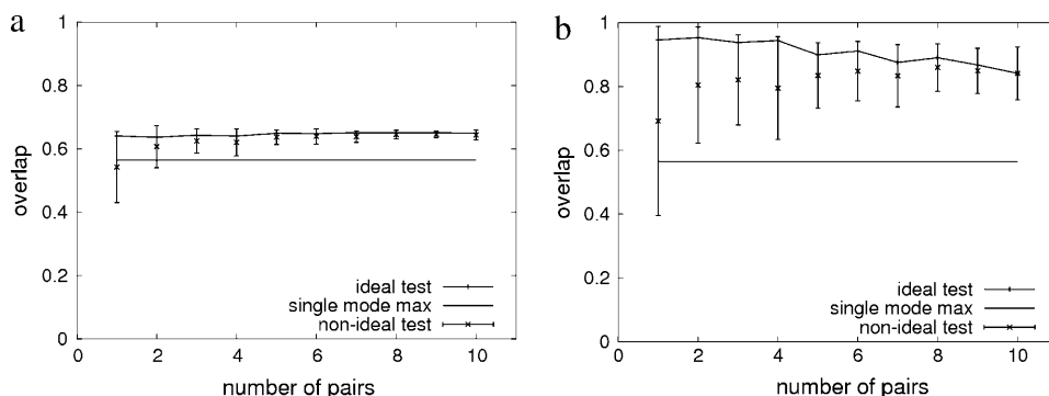
FIGURE 2 Summary of results for transition (1ddt → 1mdt). Panel a shows the overlap between the computed and the measured conformational changes versus the number of pairwise distance constraints. Panel b shows the overlap between the computed conformational change and mode No. 2 versus the number of pairwise distance constraints. Line with pluses, result for the ideal test; horizontal line, the maximal overlap between any single mode and the measured conformational change; x-marks with error bars, result for the nonideal test 1, where the error bar shows 1 SD.
